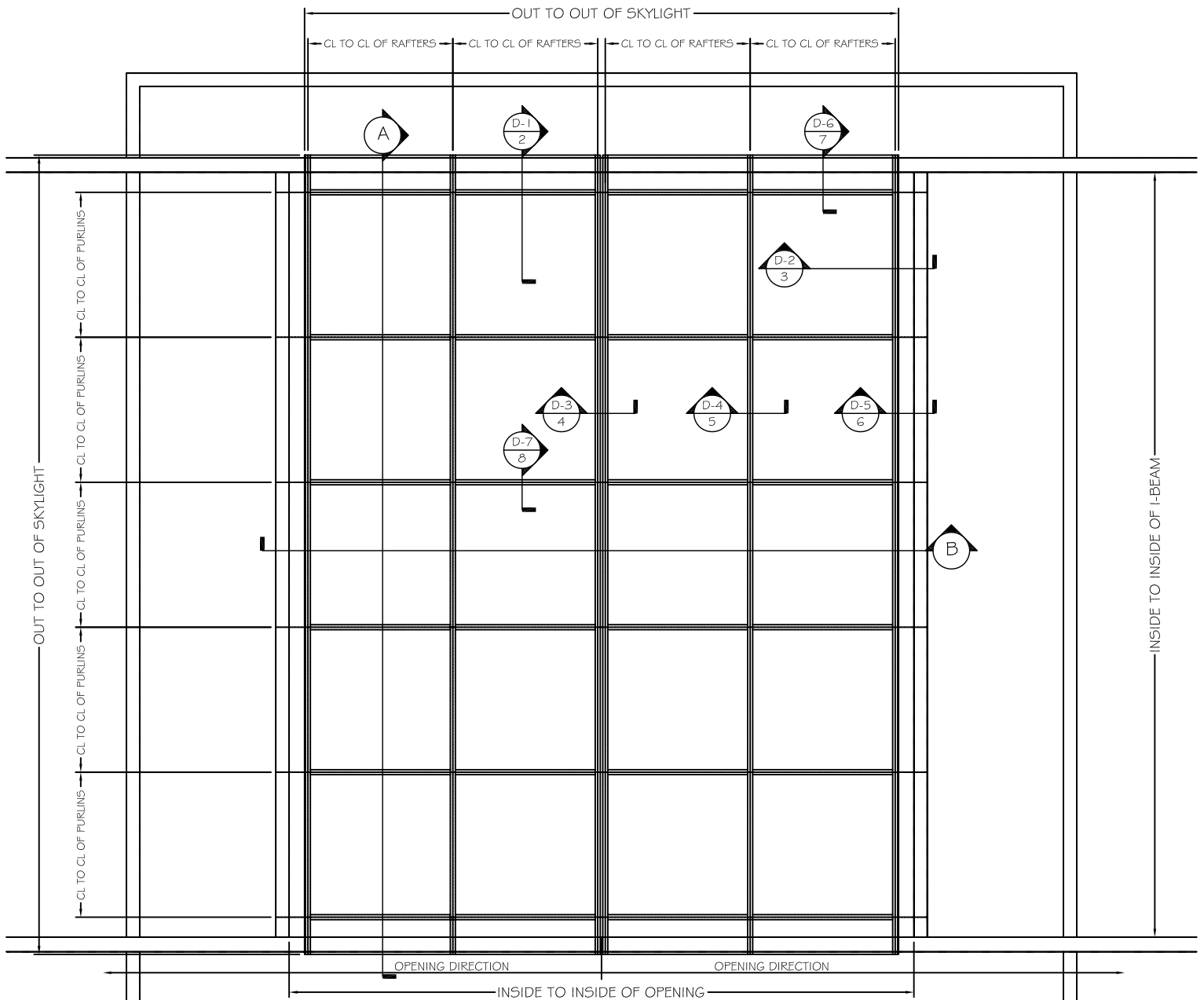
SKYLIGHT PLAN
